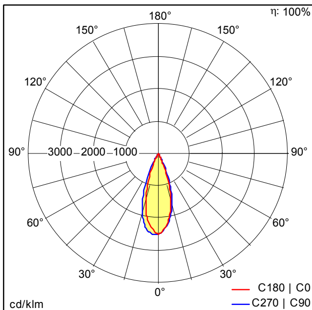
TE_LILY_LED_SPOT_IP44_38_68_850_940.ltd
