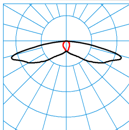
LIQ 50N-SB3L-LR/1350-740 2G1 ET (CLO end value) TX277914 ■ C0 - C180 ■ C90 - C270 DIN 5040: A30 UTE: 1,00 l CEN Flux Code: 31 64 92 100 100
