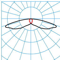
LIQ 50N-SB3L-LR/1350-740 2G1 ET (CLO initial value) TX278256 ■ C0 - C180 ■ C90 - C270 DIN 5040: A30 UTE: 1,00 l CEN Flux Code: 31 64 92 100 100
