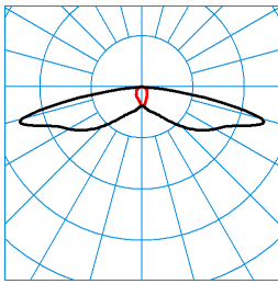
Jovie 50-SB3L-LR/1350-740 2G1 ET (CLO initial value) TX301366 ■ C0 - C180 ■ C90 - C270 DIN 5040: A20 UTE: 1,00 l CEN Flux Code: 29 61 91 100 100
