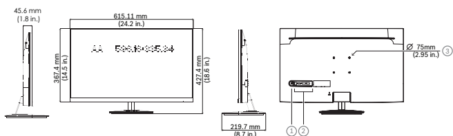
Fig. 1: Dimensions moniteur LED hautes performances (27")
