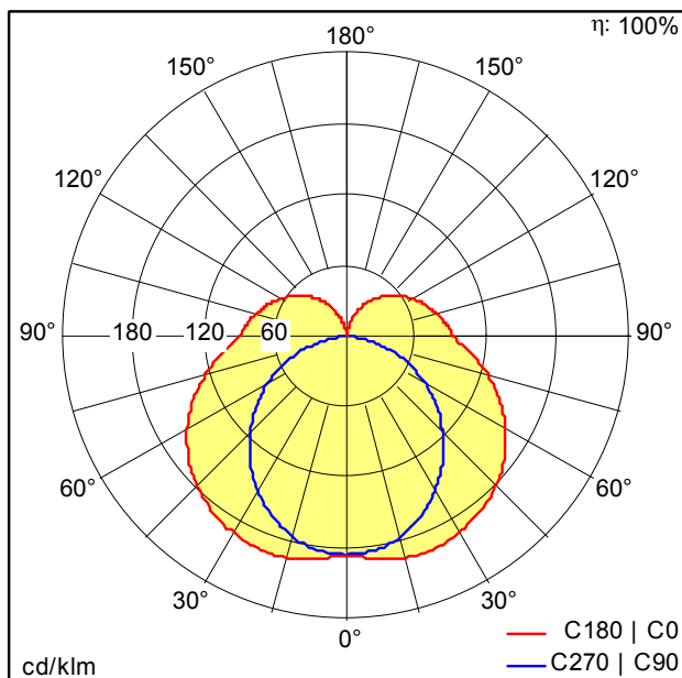
D39715AA_LINARIA_LED3700-840_L1508_PM_WH.Idt
