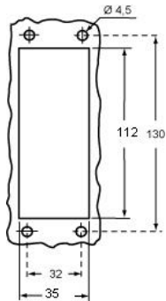
Catalogue drawings
