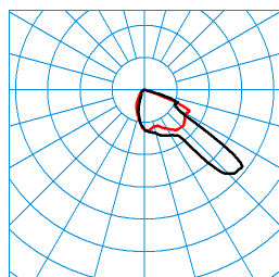
LIQ 50N-FR1L/5600-727 6G1 ET (CLO initial value) TX278094 ■ C0 - C180 ■ C90 - C270 DIN 5040: A40 UTE: 1,00 F CEN Flux Code: 41 83 99 100 100
