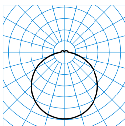
Olisq Act RWD3 DW 30 ETBLE +CAS IP54 + Olisq RWD3 ZDR 1/2 01 (ACTDWW) TX565592
