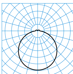
Olisq Act RWD3 DW 30 ETBLE +CAS IP54 + Olisq RWD3 ZDR 1/2 03 (ACTDWW) TX565595
