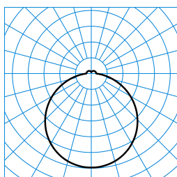
Olisq Act RWD3 DW 30 ETBLE +CAS IP54 (ACTDSU) TX565579
