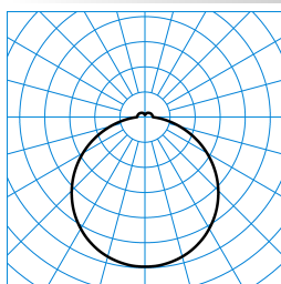
Olisq Act RWD3 DW 30 ETBLE +CAS IP54 (ACTDWW) TX565580
