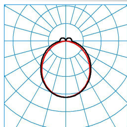
ELINE FL HE+ DSL160 830 L225 1 20
