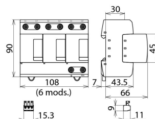
Dimensions DV M TNC 255 (FM)
