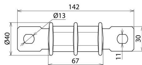
Dimensions DSFS
