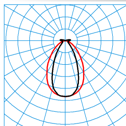
AragF 15 P-N 80-840 +LLWRC PC TX112904
