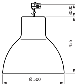
CustomCreate PT520T
