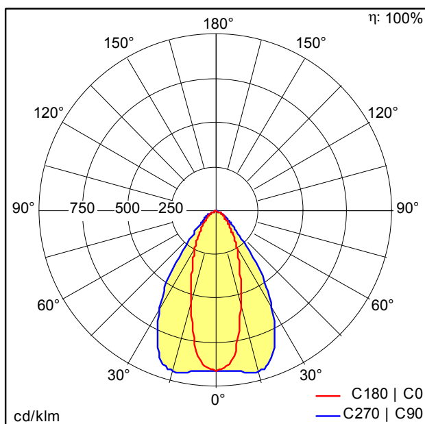
D46663_CR2PL_M25k-840_PM_NB_LDO.ltd
