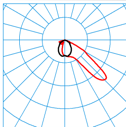
Jovie 50I-AM2L-MLLR/16-42-740 4G1 ETDD (CLO end value) ■ C0 - C180 TX264157 ■ C90 - C270 DIN 5040: A40 UTE: 1,00 F CEN Flux Code: 47 91 100 100 100
