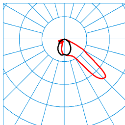
Jovie 50I-AM2L-MLLR/16-42-740 4G1 ETDD (CLO initial value) ■ C0 - C180 TX264156 ■ C90 - C270 DIN 5040: A40 UTE: 1,00 F CEN Flux Code: 47 91 100 100 100
