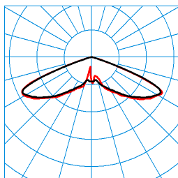
Publisca P1W-RB6L-LRA/2600-740 3G1S ET (CLO initial value) TX300517 ■ CO - C180 ■ C90 - C270 DIN 5040: A20 UTE: 1,00 J CEN Flux Code: 19 57 99 100 100 0 50 50 0
