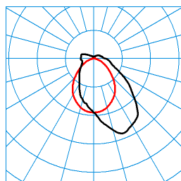
TugraHE 12 PAW 24-75/16ML-840 ET PC 23 (STAG13) TX425105 ■ C0 - C180 ■ C90 - C270 DIN 5040: B40 UTE: 0,86 E + 0,14 T CEN Flux Code: 48 77 92 86 100 13 32 64 14
