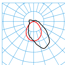
TugraHE 12 PAW 24-75/16ML-840 ET PC 23 (STAG14) TX425232 ■ C0 - C180 ■ C90 - C270 DIN 5040: B40 UTE: 0,86 E + 0,14 T CEN Flux Code: 48 77 92 86 100 13 32 64 14
