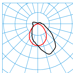
TugraHE 12 PAW 24-75/16ML-840 ET PC 23 (STAG12) TX425234 ■ C0 - C180 ■ C90 - C270 DIN 5040: B40 UTE: 0,86 E + 0,14 T CEN Flux Code: 48 77 92 86 100 13 32 64 14
