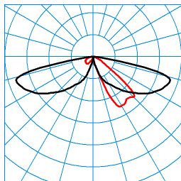
LTX P-AB2L-LRA/15/18/26-730 4G1 (2600 lm) TX062700 ■ C0 - C180 ■ C90 - C270 DIN 5040: A20 UTE: 1,00 l CEN Flux Code: 24 61 92 100 100 0 0 0 0
