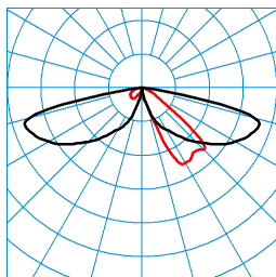
LTX P-AB2L-LRA/15/18/26-730 4G1 (1500 lm) TX059698 ■ C0 - C180 ■ C90 - C270 DIN 5040: A20 UTE: 1,00 l CEN Flux Code: 24 61 92 100 100 0 0 0 0
