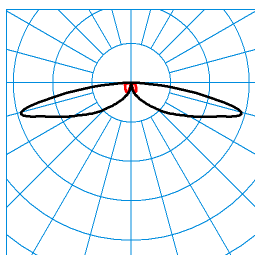
CS 19 100-SB3L/2900-730 2G1S ETDD (CLO initial value) TX300152 ■ C0 - C180 ■ C90 - C270 DIN 5040: A20 UTE: 1,00 J CEN Flux Code: 22 52 84 100 100 0 0 0 0
