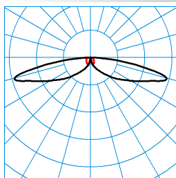
CS 19 100-SB3L/2900-730 2G1S ETDD (CLO end value) TX300151 ■ C0 - C180 ■ C90 - C270 DIN 5040: A20 UTE: 1,00 J CEN Flux Code: 22 52 84 100 100 0 0 0 0
