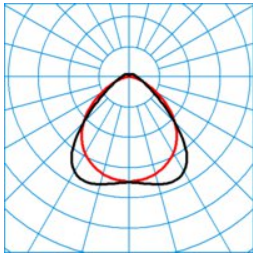
7850 HE PW40-120 ML 830 L150 14 50 ■ C0 - C180 DIN 5040 = A40 CEN flux code = 56 85 95 93 100 15 39 67 7 UGR I 3 = 24,4 UGR q 3 = 23,0 UTE 3 = 0.93 D + 0.07 T
