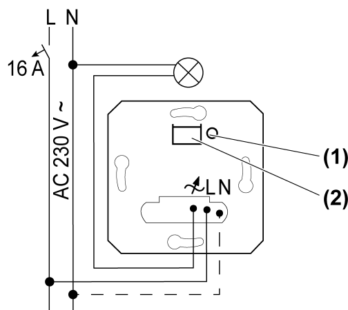
Figure 1: Schéma de raccordement
