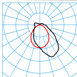
TugraHE 18 PAW 68-110/16ML-840 ET PC 23 (STAG10) TX425239 C0 - C180 C90 - C270 DIN 5040: B40 UTE: 0,86 E + 0,14 T CEN Flux Code: 48 77 92 86 100 13 32 64 14
