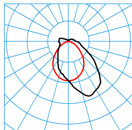
TugraHE 18 PAW 68-110/16ML-840 ET PC 23 (STAG12) TX425259 C0 - C180 C90 - C270 DIN 5040: B40 UTE: 0,86 E + 0,14 T CEN Flux Code: 48 77 92 86 100 13 32 64 14
