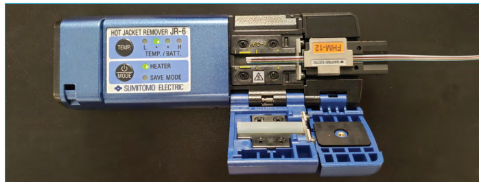
Figure 7: Removing the jacket from the fiber.
