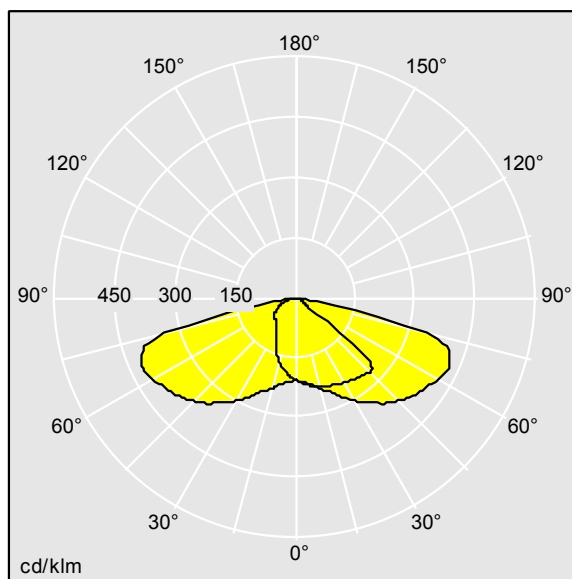
TL_CQS36L70NR740.ltd
