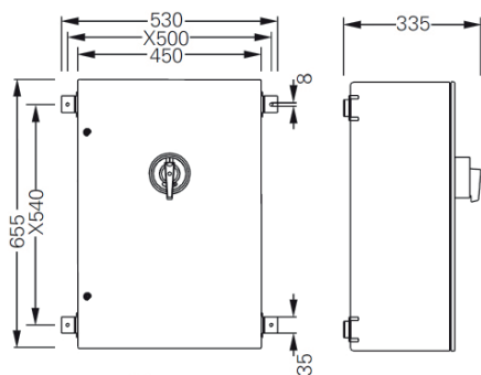
EXKO 2247..., 125 A 6-polig EXKO 2247..., 180 A 6-polig
