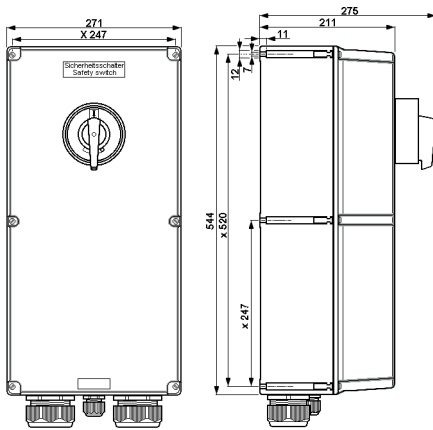
GHG 265..., 125 A 3- / 4-pole GHG 266 ..., 180 A 3-pole
