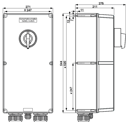
GHG 265..., 125 A 3- / 4-polig GHG 266 ..., 180 A 3-polig
