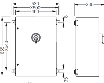
EXKO 2247..., 125 A 6-pole EXKO 2247..., 180 A 6-pole
