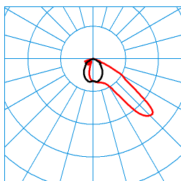
Jovie 50I-AM2L-LRA/4200-740 4G1 ET (CLO end value) TX301363 ■ C0 - C180 ■ C90 - C270 DIN 5040: A40 UTE: 1,00 F CEN Flux Code: 47 91 100 100 100
