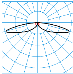
CS 19 100-SB3L-SLR1/2200-740 2G1S ET (CLO end value) TX300157 ■ C0 - C180 ■ C90 - C270 DIN 5040: A20 UTE: 1,00 J CEN Flux Code: 22 52 84 100 100 0 0 0 0
