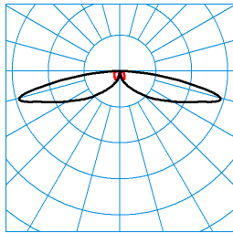
CS 19 100-SB3L-SLR1/2200-740 2G1S ET (CLO initial value) TX300158 ■ C0 - C180 ■ C90 - C270 DIN 5040: A20 UTE: 1,00 J CEN Flux Code: 22 52 84 100 100 0 0 0 0
