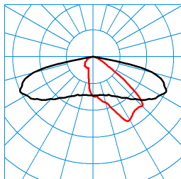
LIQ 50N-AB2L-LR/1350-740 2G1 ET (CLO initial value) TX277676 ■ C0 - C180 ■ C90 - C270 DIN 5040: A30 UTE: 1,00 G CEN Flux Code: 34 71 96 100 100 0 0 0 0
