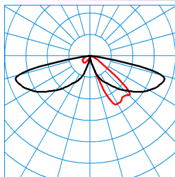
LTX L-AB2L-LRA/15/18/26-730 4G1 (1800 lm) TX061510 ■ C0 - C180 ■ C90 - C270 DIN 5040: A20 UTE: 1,00 l CEN Flux Code: 24 61 92 100 100 0 0 0 0
