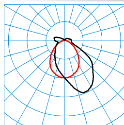
TugraHE Act 21 PAW 80-840 ETDD8 01 (ACTDWW) TX303517 ■ C0 - C180 ■ C90 - C270 DIN 5040: B40 UTE: 0,87 E + 0,13 T CEN Flux Code: 48 79 93 87 100 7 25 60 13
