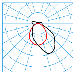
TugraHE Act 21 PAW 80-840 ETDD8 01 (ACTDCW) TX303413 ■ C0 - C180 ■ C90 - C270 DIN 5040: B40 UTE: 0,87 E + 0,13 T CEN Flux Code: 48 79 93 87 100 7 25 60 13
