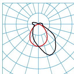
TugraHE Act 21 PAW 80-840 ETDD8 01 (ACTDSU) TX302550 ■ C0 - C180 ■ C90 - C270 DIN 5040: B40 UTE: 0,87 E + 0,13 T CEN Flux Code: 48 79 93 87 100 7 25 60 13
