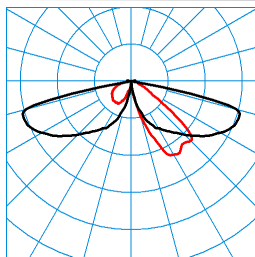
CS 19 100-AB2L-LR/3800-740 4G1S ET (CLO end value) TX300028 ■ C0 - C180 ■ C90 - C270 DIN 5040: A20 UTE: 1,00 l CEN Flux Code: 27 65 96 100 100 0 0 0 0
