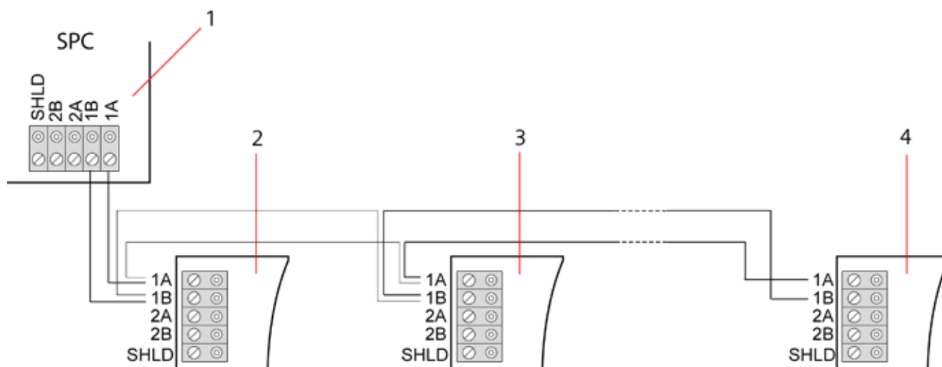
Configuration multipoint
