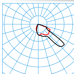
LIQ 50N-FR1L/5600-730 6G1 ET (CLO end value) TX277800 ■ C0 - C180 ■ C90 - C270 DIN 5040: A40 UTE: 1,00 F CEN Flux Code: 41 83 99 100 100
