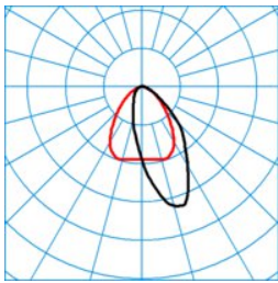
7850 HE LAN60 827 L150 2 50 ■ C0 - C180 DIN 5040 = A50 CEN flux code = 63 89 98 98 100 0 6 44 2 UGR 1 = 0,0 UGR q = 0,0 UTE = 0.98 C + 0.02 T
