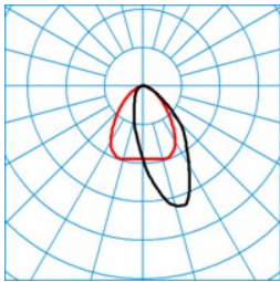
7850 HE LAN60 865 L150 3 50 ■ C0 - C180 DIN 5040 2 = A50 CEN flux code = 63 89 98 98 100 0 6 44 2 UGR 1 2 = 0,0 UGR q 2 = 0,0 UTE 2 = 0.98 C + 0.02 T
