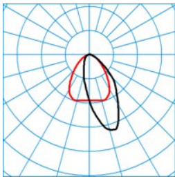
7850 HE LAN60 840 L150 4 50 ■ C0 - C180 DIN 5040 3 = A50 CEN flux code = 63 89 98 98 100 0 6 44 2 UGR 1 3 = 0,0 UGR q 3 = 0,0 UTE 3 = 0.98 C + 0.02 T
