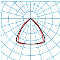
7850 HE LW22100 840 L225 4 50 ■ C0 - C180 DIN 5040 3 = A50 CEN flux code = 77 97 99 99 100 0 0 38 1 UGR 1 3 = 20,3 UGR q 3 = 18,9 UTE 3 = 0.99 B + 0.01 T
