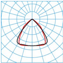
7850 HE LW22100 865 L225 3 50 ■ C0 - C180 DIN 5040 2 = A50 CEN flux code = 77 97 99 99 100 0 0 38 1 UGR 1 2 = 20,4 UGR q 2 = 19,1 UTE 2 = 0.99 B + 0.01 T
