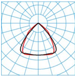
7850 HE LW22100 827 L225 2 50 ■ C0 - C180 DIN 5040 = A50 CEN flux code = 77 97 99 99 100 0 0 38 1 UGR 1 = 20,3 UGR q = 18,9 UTE = 0.99 B + 0.01 T
