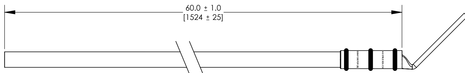
FACTORY CRIMPED #4 AWG COMMON BONDING NETWORK (CBN) JUMPER WIRE ASSEMBLY (QTY. 1) INCLUDES: LCC4-14JAWH (QTY. 1) #4 AWG [21.2mm 2 ] WIRE - GREEN/YELLOW INSULATION 60" [1524] LONG
