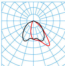
Jovie 70I-AM3L/18000-740 18G1 ETDD (CLO initial value) TX301890 ■ C0 - C180 ■ C90 - C270 DIN 5040: A50 UTE: 1,00 D CEN Flux Code: 59 89 100 100 100
