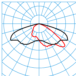
LIQ 70N-AB7L-SLR1/9100-740 10G1 ET (CLO initial value) TX277809 ■ C0 - C180 ■ C90 - C270 DIN 5040: A30 UTE: 1,00 G CEN Flux Code: 35 73 98 100 100 0 0 0 0
