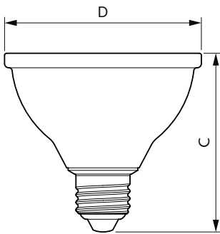
MAS LEDspot CLA D 9.5-75W 840 PAR30S 25D
