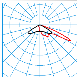
LnPlus 60-AM19L/24000-730 18G1 ETDD (CLO end value) TX377259
