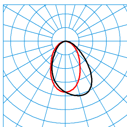
ArimoFit G2 Act D3 D-WW 53-8 ETDD8 01/01 (ACTDCW) TX377936 ■ C0 - C180 ■ C90 - C270 DIN 5040: A50 UTE: 1,00 C CEN Flux Code: 61 87 98 100 100 0 0 0 0
