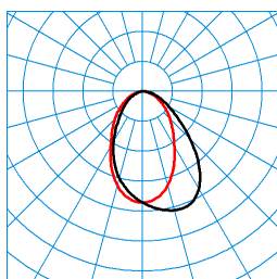
ArimoFit G2 Act D3 D-WW 53-8 ETDD8 01/01 (ACTDSU) TX377467 ■ C0 - C180 ■ C90 - C270 DIN 5040: A50 UTE: 1,00 C CEN Flux Code: 61 87 98 100 100 0 0 0 0
