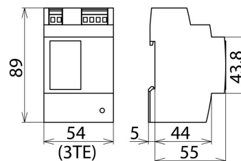
Dimensions PSU DC24 30W
