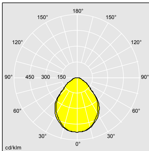
D44261AA_EQL_840_HF_L2000_LRO_SR_.ldt
