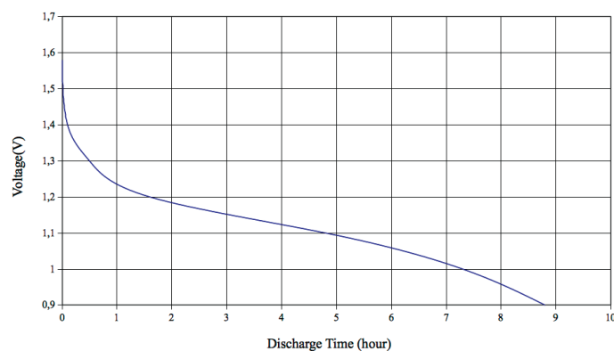
3.9Ω 1hour/day Discharge Curve
