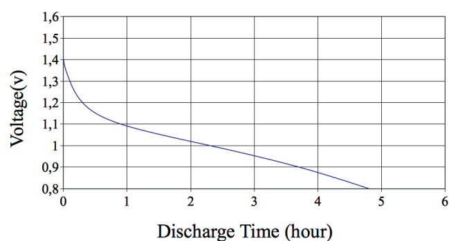
2.2Ω 1hour/day Discharge Curve
