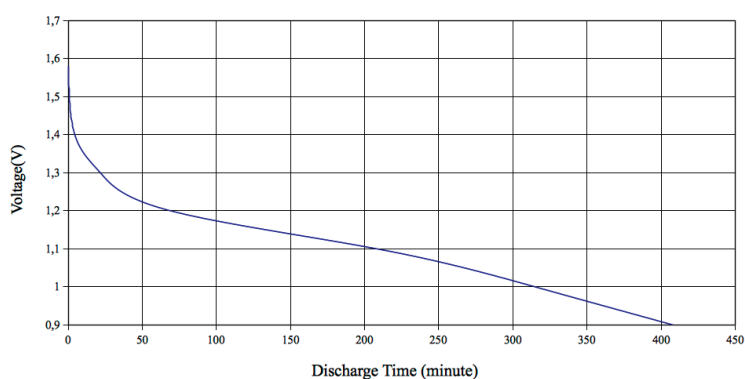
3.9Ω Continuous Discharge Curve
