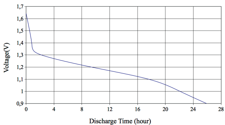
10Ω 4hour/day Discharge Curve
