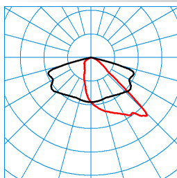
Cuvia 60-AB6L-LR/5100-740 8G1S TX047063 ■ C0 - C180 ■ C90 - C270 DIN 5040: A30 UTE: 1,00 E CEN Flux Code: 40 75 98 100 100
