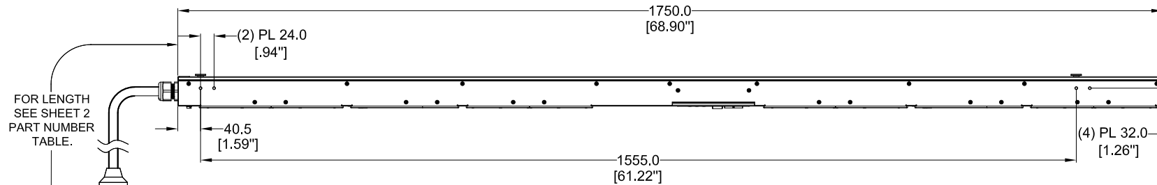
RIGHT VIEW
