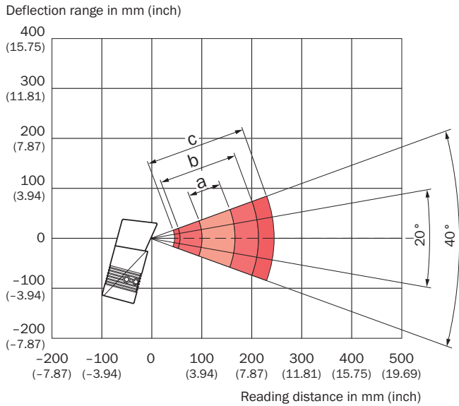
Resolution a: 0.20 mm (7.9 mil) b: 0.35 mm (13.8 mil) c: 0.50 mm (19.7 mil) ① Diagram applies to focus position of 140 mm
