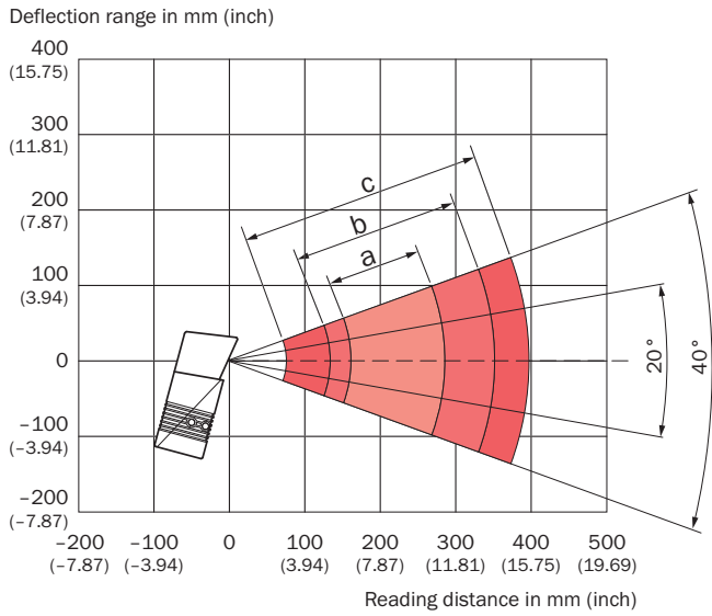
Resolution a: 0.25 mm (9.8 mil) b: 0.35 mm (13.8 mil) c: 0.50 mm (19.7 mil) ① Diagram applies to focus position of 215 mm
