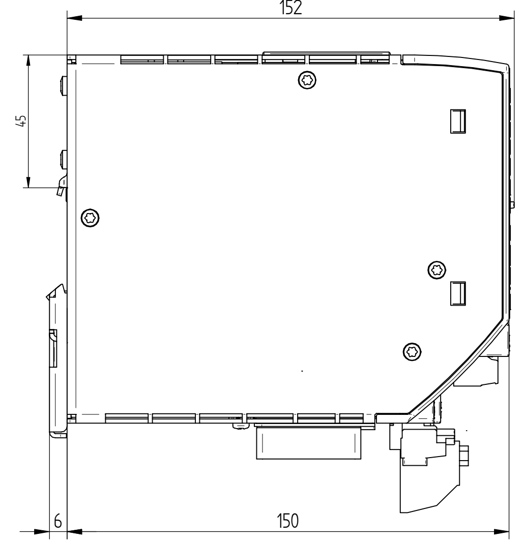
Links / Left
