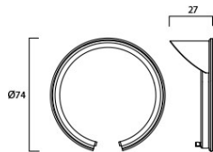
Dimensions (mm)
