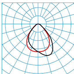
ArimoFit G2 Act D2 P-WW 42-8 ETDD8 01/01 (ACTDCW) TX377064 ■ C0 - C180 ■ C90 - C270 DIN 5040: A50 UTE: 1,00 C CEN Flux Code: 66 90 97 100 100
